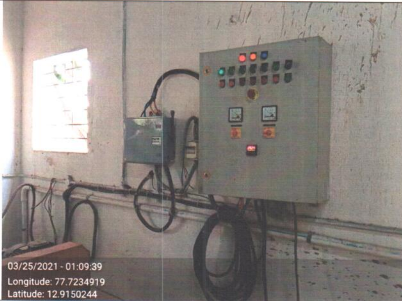
Power Distribution for STP Plant
